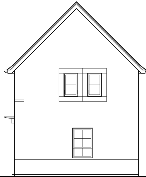
FRONT ELEVATION Ennerdale
